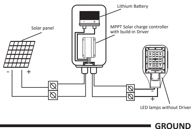
Parts Connection Diagram
